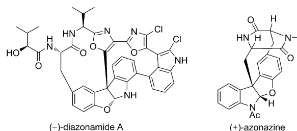
Figure 1. Representative benzofuroindoline natural products. Ac = acetyl.
