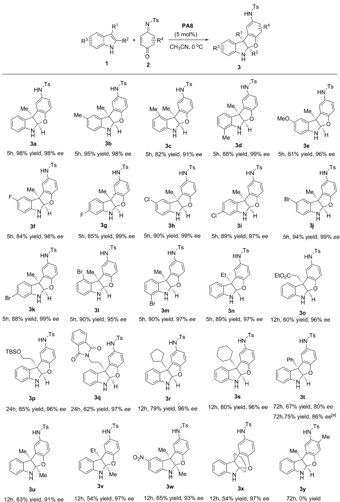
Scheme 1. Substrate scope. Reaction conditions: Unless otherwise specified, the reactions were carried out with 0.20 mmol of 1 , 0.30 mmol of 2 , and 0.01 mmol of PA8 in 2 mL of acetonitrile at 0 °C. Yields shown are of the isolated products and based on 1 . Enantiomeric excesses were determined by HPLC analysis on a chiral stationary phase. [a] 10 mol % of PA8 was employed. TBS = tert -butyldimethylsilyl.
